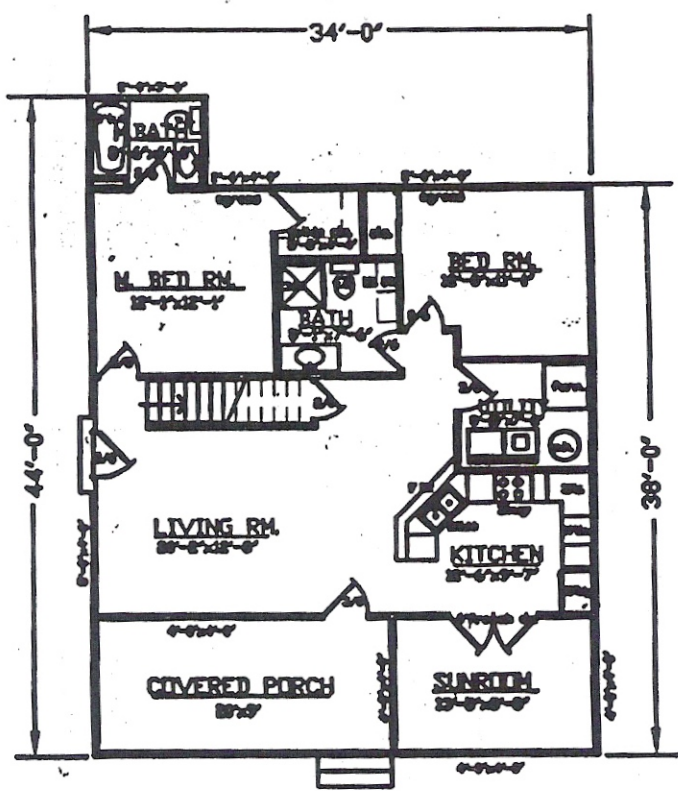
FIRST FLOOR PLAN 1160 sq. ft.
